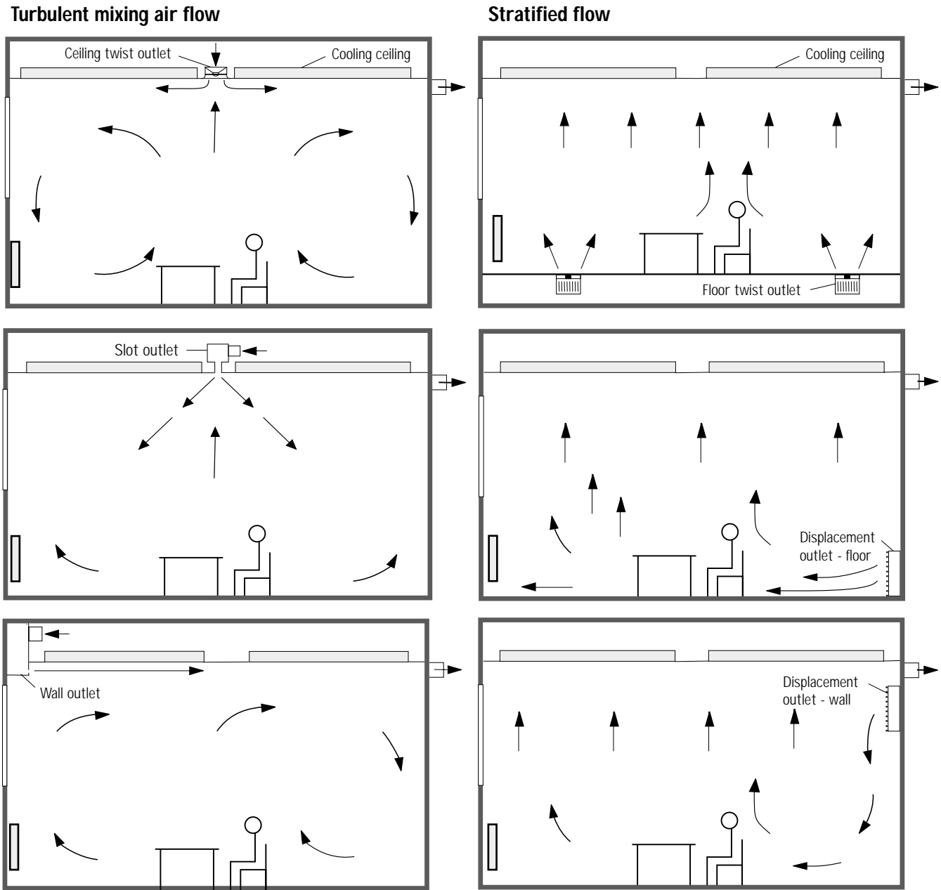
Figure 3: Combination of cooling ceilings with different air distribution systems
